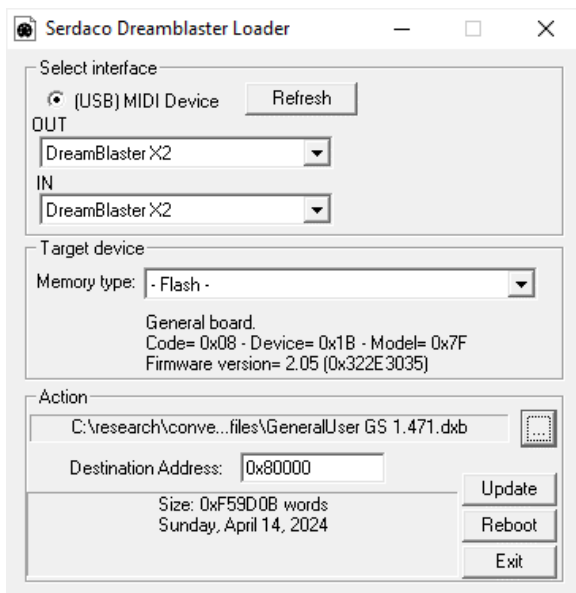
Figure 25: X2Upload : Bank file chosen.
