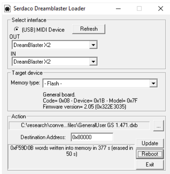
Figure 27: X2Upload : Upload ready
