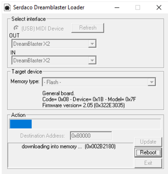
Figure 26: X2Upload : downloading into memory
